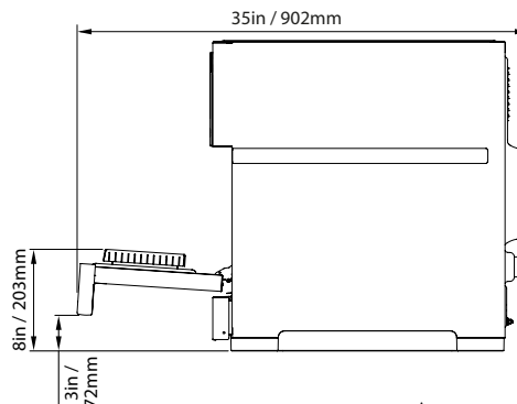
Dimensional drawings apply to "Classic" exterior
